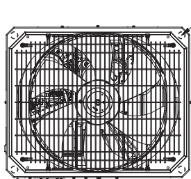
Airguide fastening total 12 places (Refer to the hole on the Airguide for the fastening position.)
