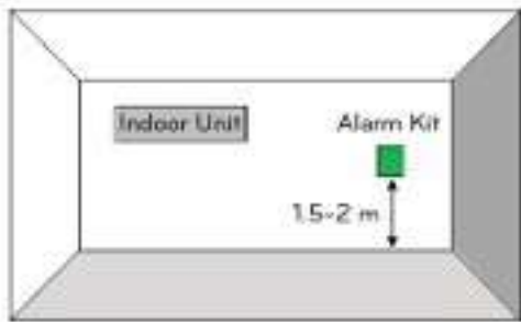
Recommendd Installation height 1.5 m ~ 2.0 m from the floor
